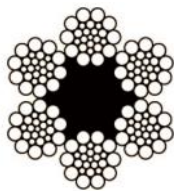
6 x 26 WARRINGTON SEAL WITH FIBER CORE
