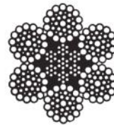
6 x 36 WARRINGTON SEAL WITH IWRC
