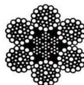
6 x 36 WARRINGTON SEALE WITH IWRC
